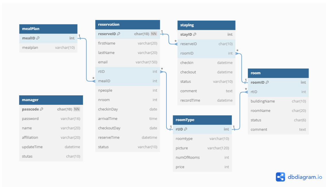
図 1 Hotel Manager ERD
