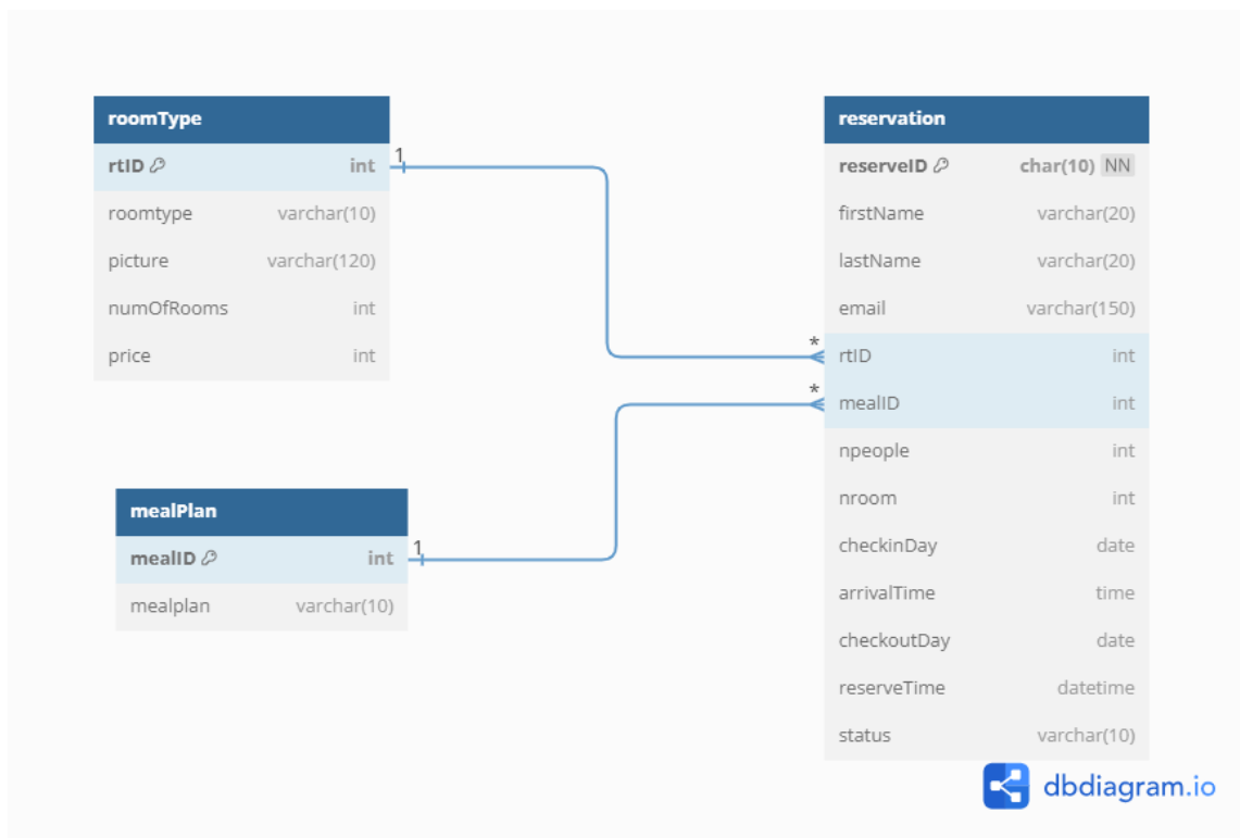
図 1 Hotel reservation ERD
